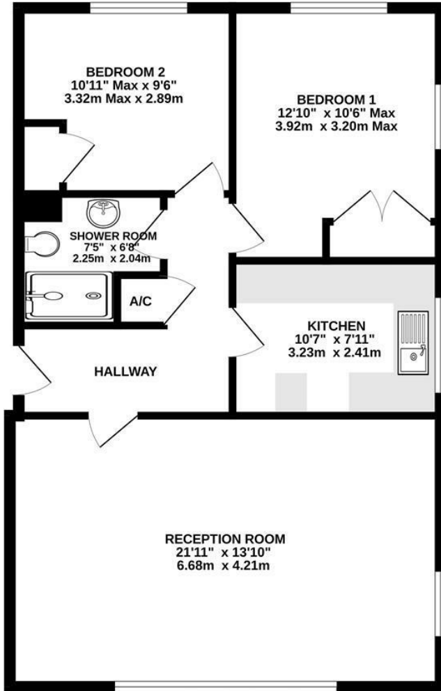
GROUND FLOOR 746 sq.ft. (69.3 sq.m.) approx.
